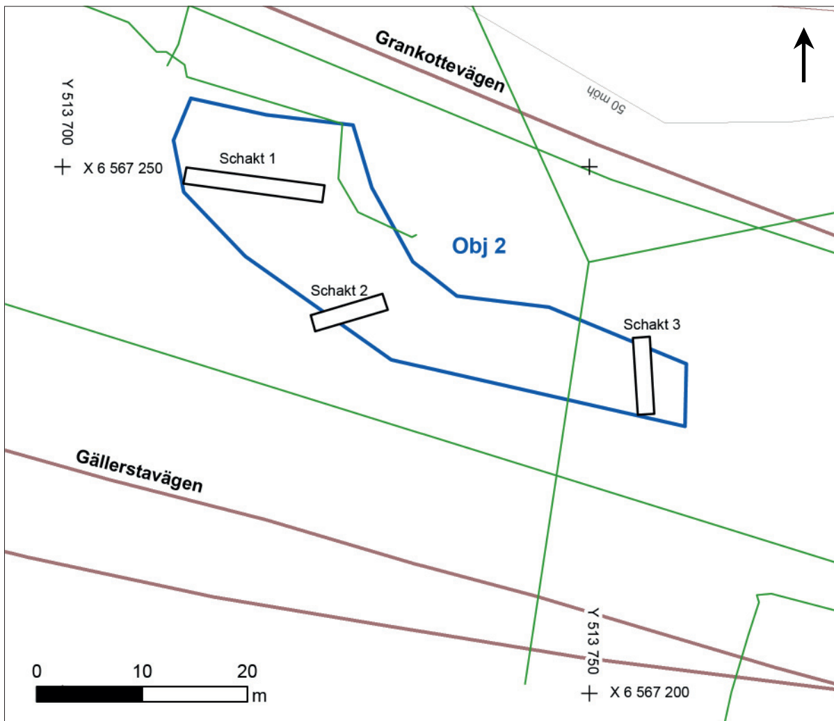
Schaktplan 1. Skala 1:500.
